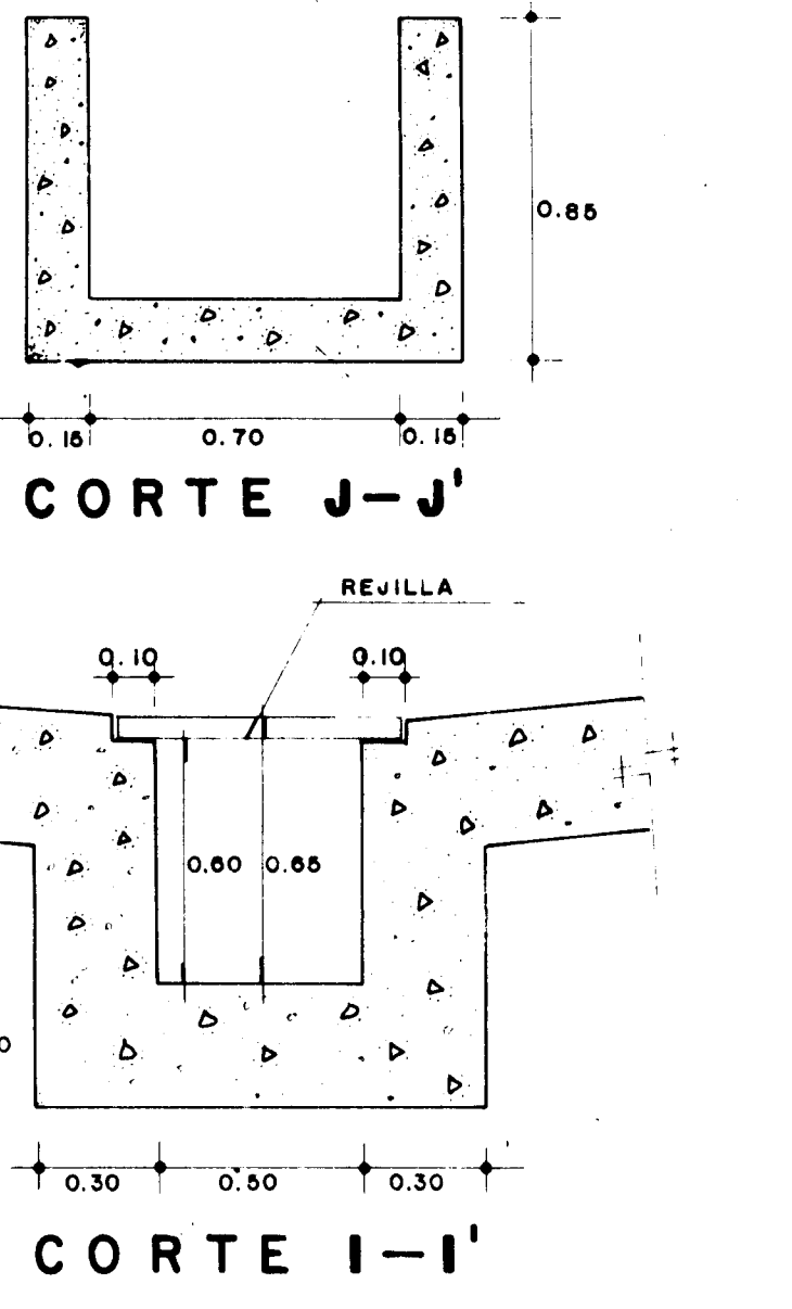
CORTE J-J' and CORTE I-I'
